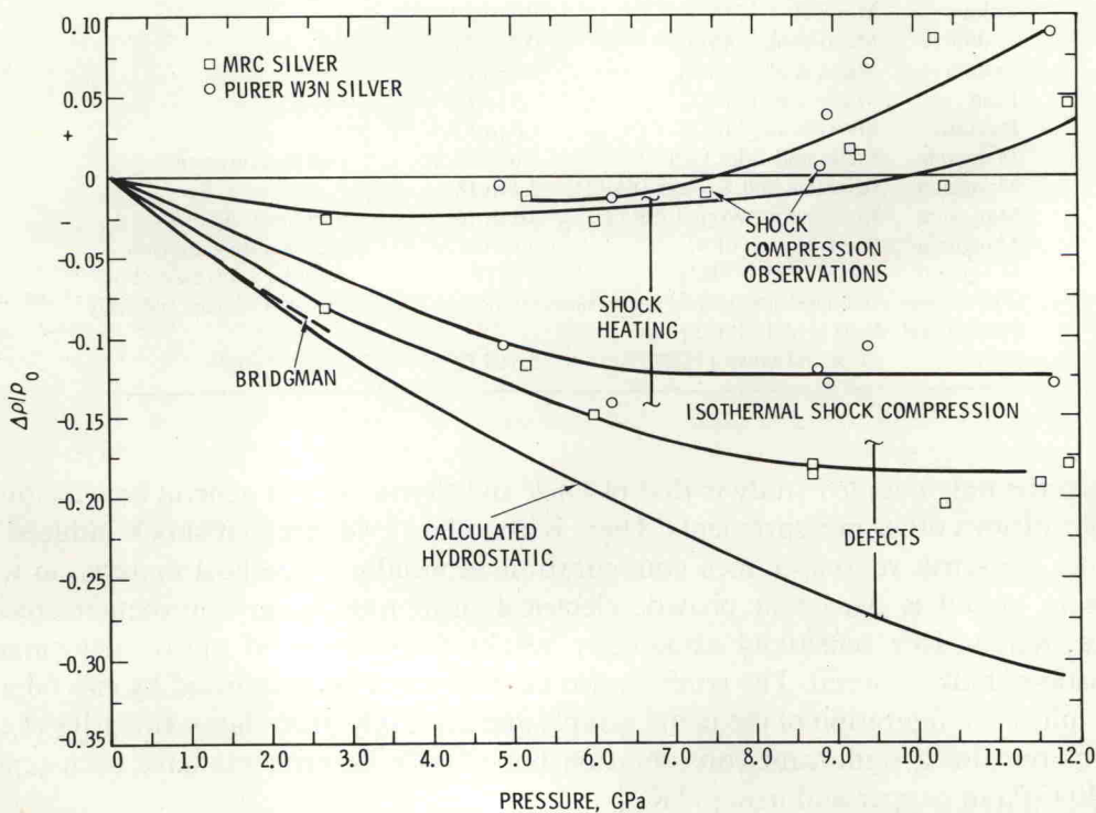
Fig. 4.10. A comprehensive study of silver under shock loading by Dick and Styris [75D1] shows evidence for resistance change due to shock-induced vacancies. The upper group of points are those observed in the shock-loading experiments. The lower group of points results from correcting those data for increases in temperature due to shock heating. The difference between the isothermal shock data and the hydrostatic predictions are evidence for resistivity change due to shock-induced vacancy concentrations of 10^{-3} per lattice site at 10 GPa.
